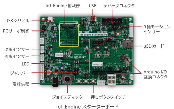
STM32L4 IoT-Engine Starter Kit
